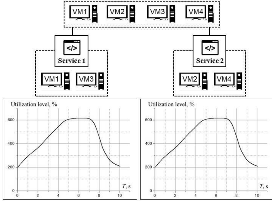
Fig. 6. Correlation-aware VMs allocations procedure
